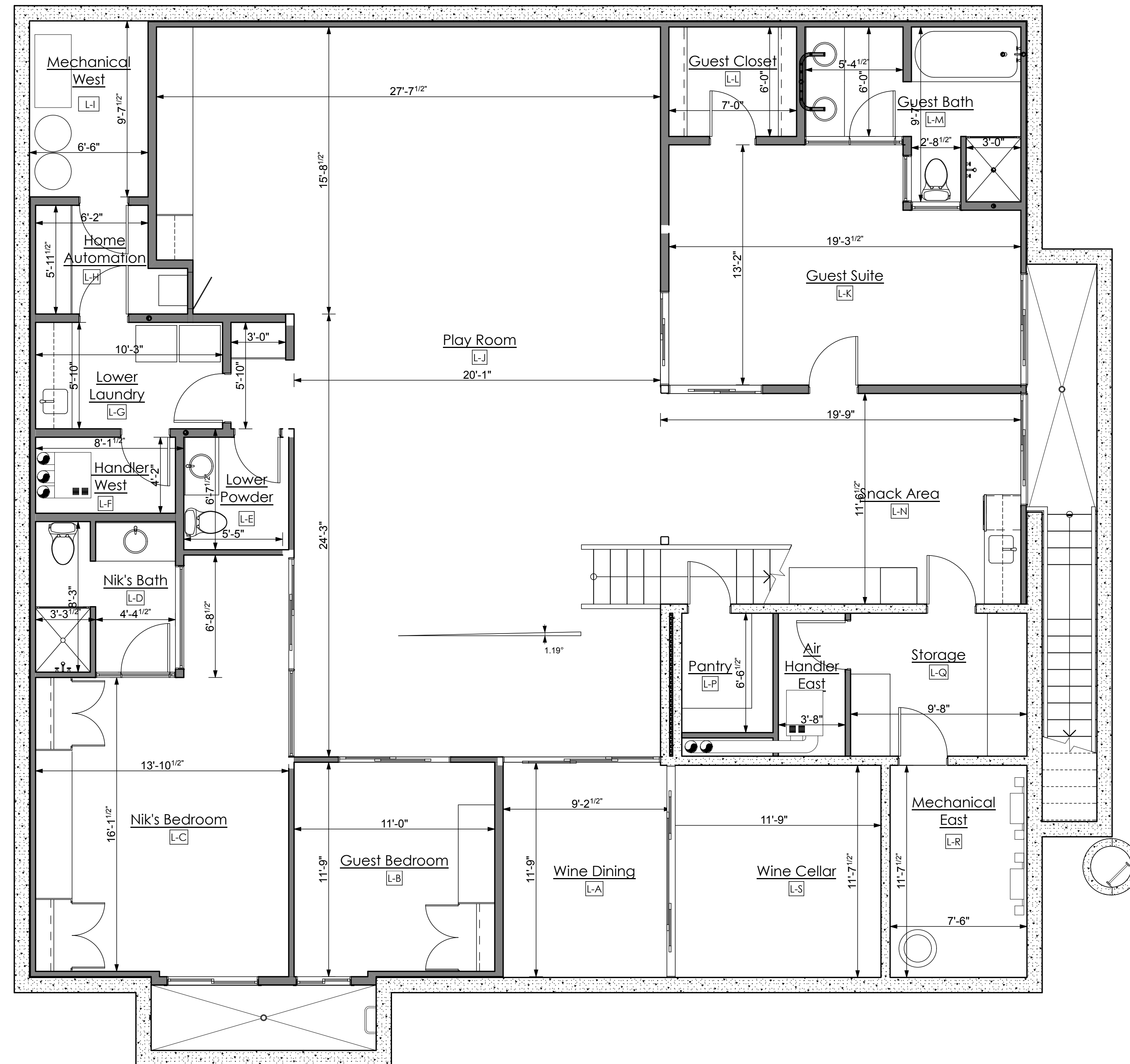
1 Overview - Basement Scale: 1/4" = 1'-0"
